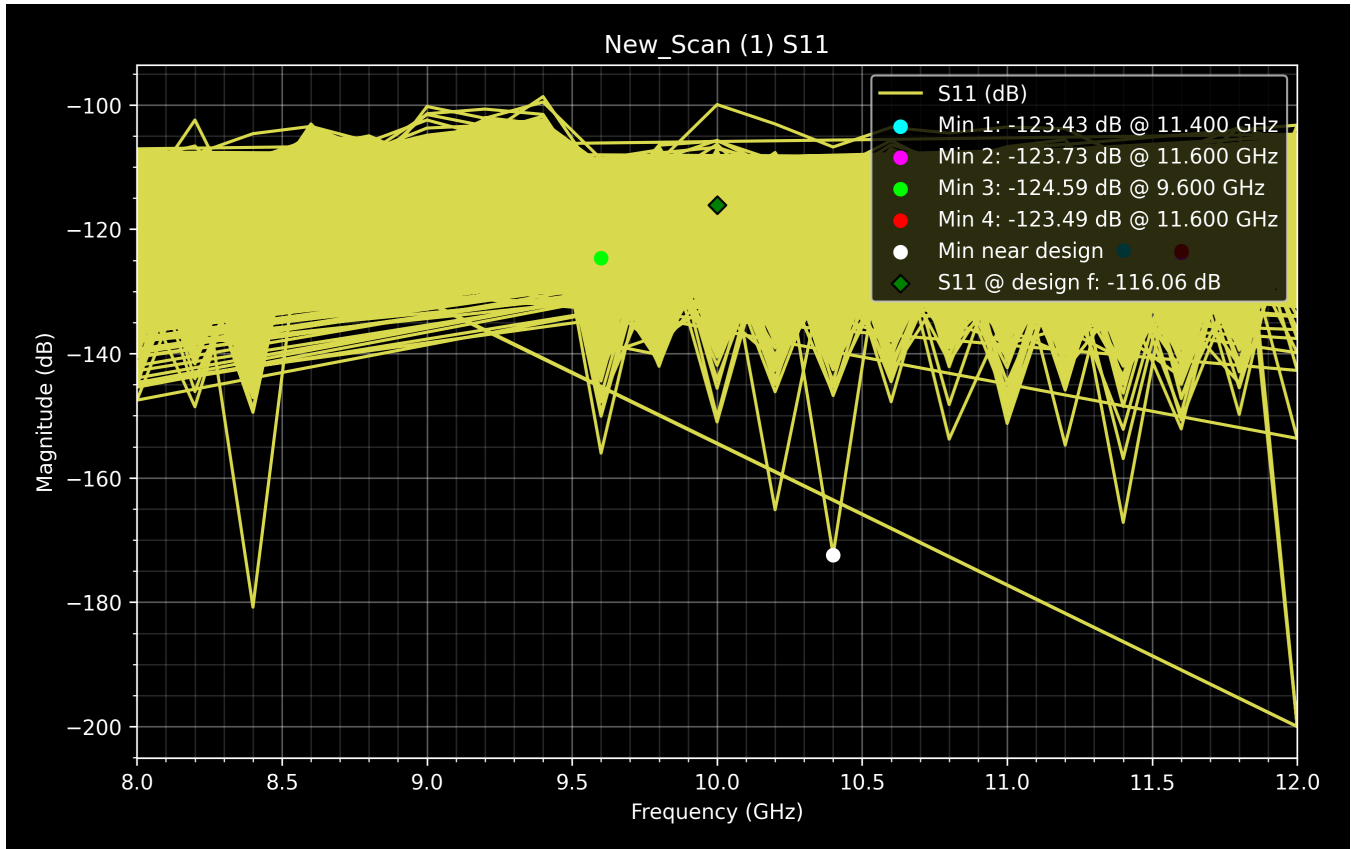
S11 Plot
